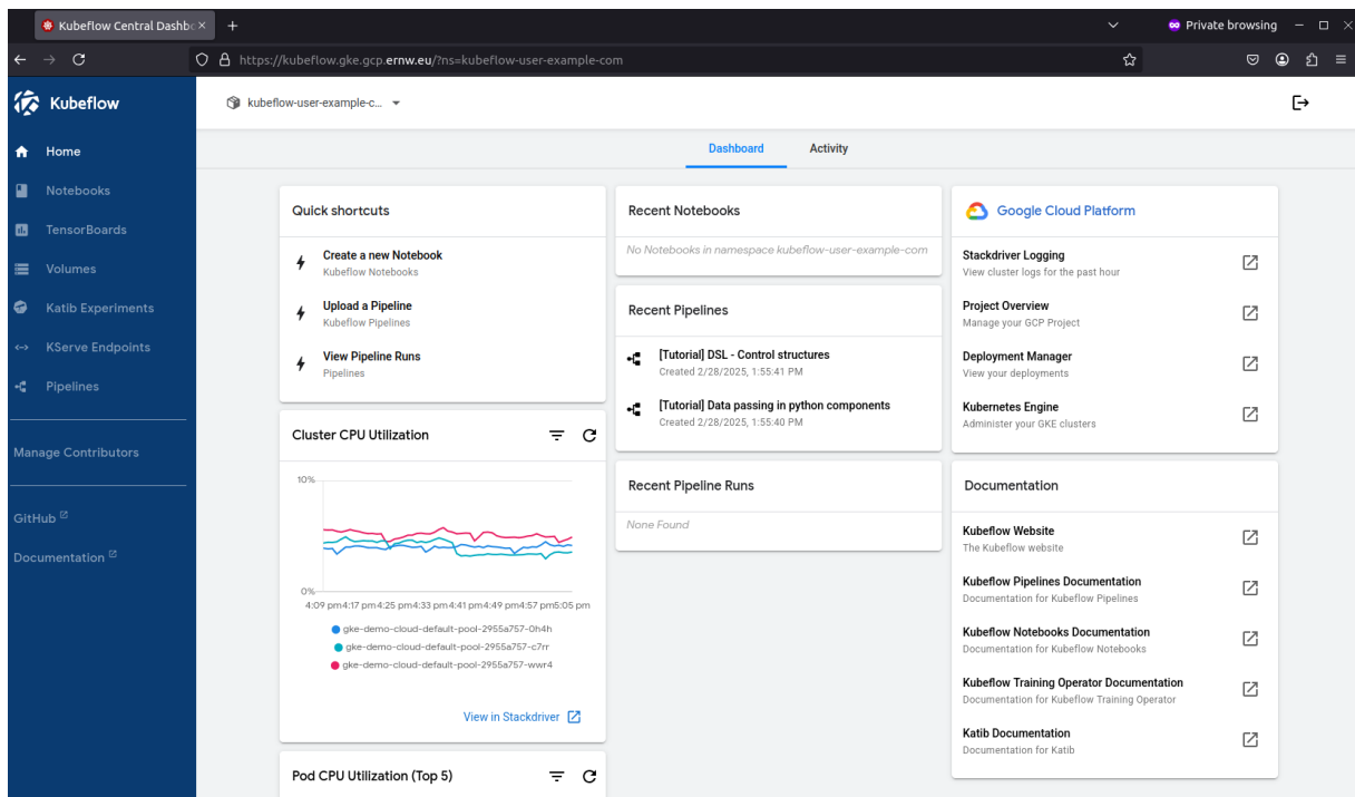
Figure 13: owned-kubeflow-instance.png
