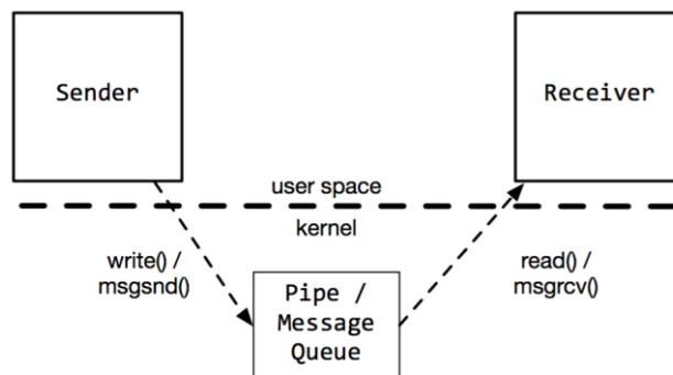
Figure 2-1: Memory copies during IPC
