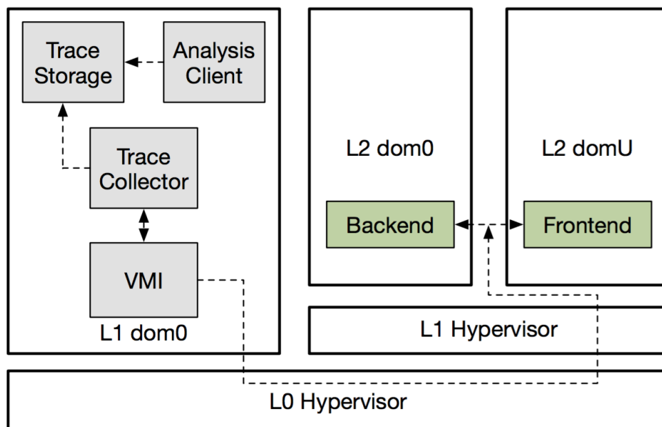
Figure 4-3. Proposed architecture
