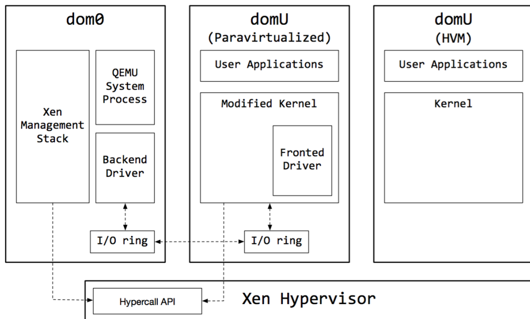
Figure 2-4. Xen architecture
