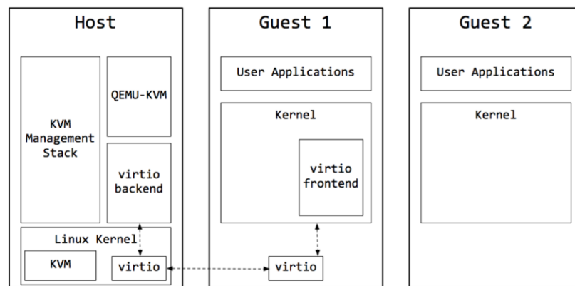
Figure 2-6. KVM architecture
