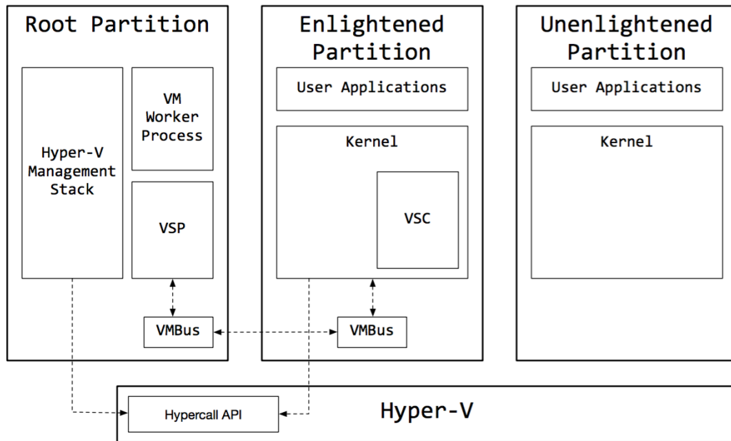
Figure 2-5. Hyper-V architecture
