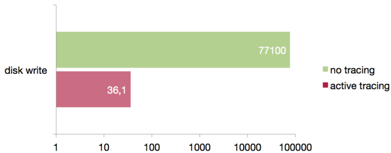
Figure 6-2. Paravirtualized disk benchmark. Write speed in KB/s.
