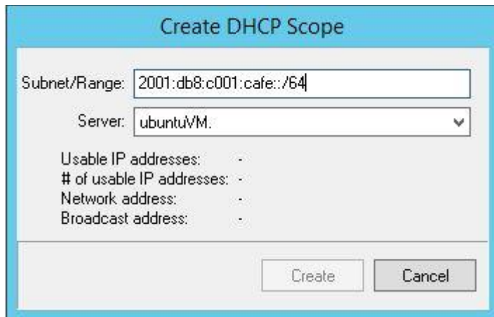
Figure 36 Missing option to create DHCPv6 scope ISC DHCP server Men&Mice
