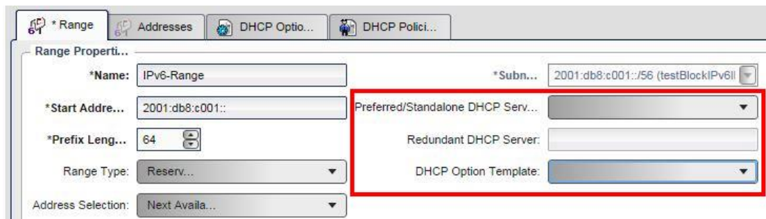
Figure 1 Missing DHCPv6 server Alcatel Lucent QIP
